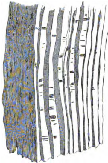
Fig. 50.—Silver-fir wood injured by mistleto. The haustoria of the latter resemble medullary rays, in the tangential and radial sections of the wood.
